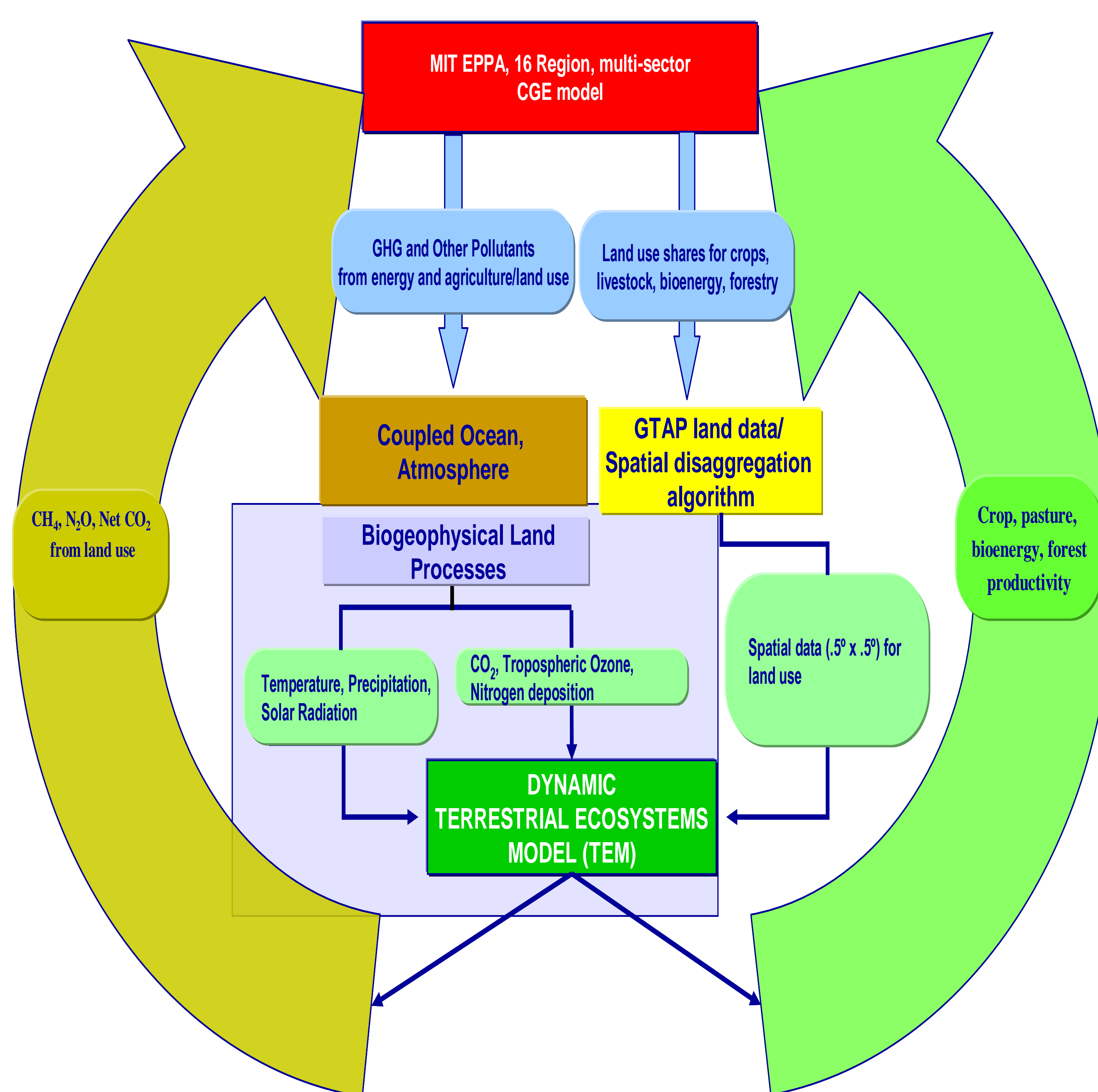
Figure 1. The EPPA model produces policy and economic scenarios that lead to changes in economic activity in all sectors of the economy, leading to changes in emissions and land use. These changes drive the atmosphere-ocean general circulation model (AOGCM) and the Terrestrial Ecosystem Model (TEM). These changes result, in turn, in feedbacks on the economic model. The linkages between the economic model, the AOGCM, and the TEM are simulated as a loosely coupled system, running EPPA to produce emissions scenarios, then the AOGCM with a reduced form version of TEM to produce climate scenarios, and then the TEM driven by climate and land use scenarios to produce productivity impacts. EPPA is then rerun with these productivity impacts, producing new scenarios of land use change, and TEM is rerun to estimate CO 2 and other trace gas impacts of the final land use scenarios. A set of six simulations are conducted considering two climate policy scenarios including a climate policy (stabilized greenhouse gas emissions at 550 ppm CO 2 -equivalent) and no-climate policy (business as usual) and three land-use and land-cover change scenarios including land use only, vegetation shift only, and land use and vegetation shift in Northern Eurasia.
