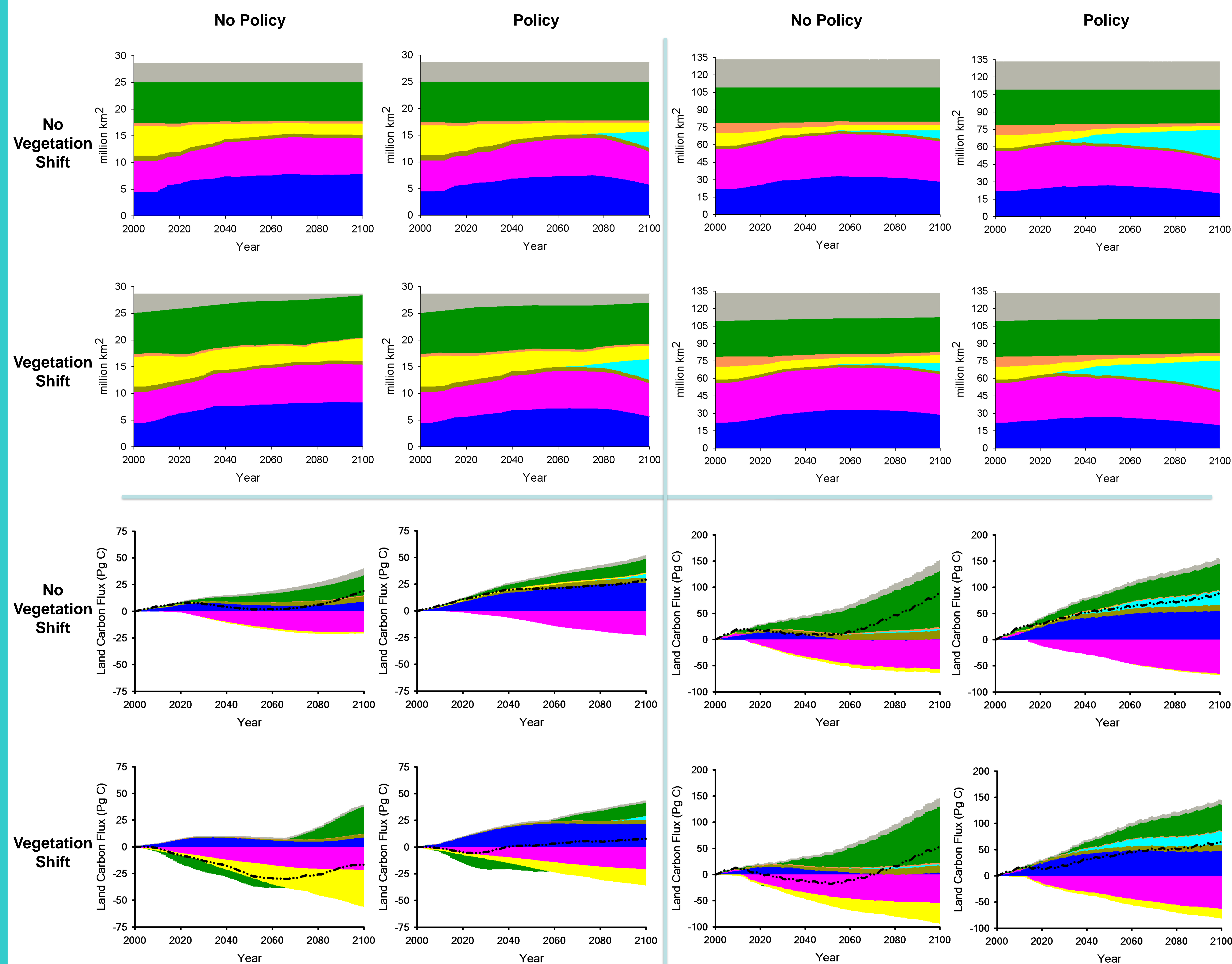
Figure 2. Land-cover and land-use change (upper panel) and land carbon flux (lower panel) in Northern Eurasia (left panel) and Global Land (right panel) over the 21 st century.
